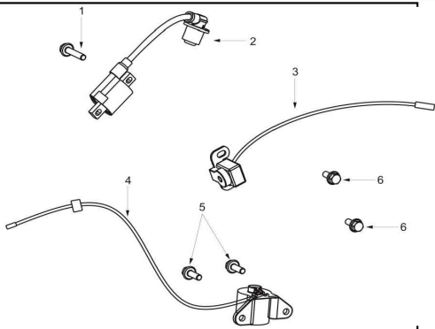
FIG.6 IGNITION COIL/WARNING DEVICE/TRIGGER COIL
