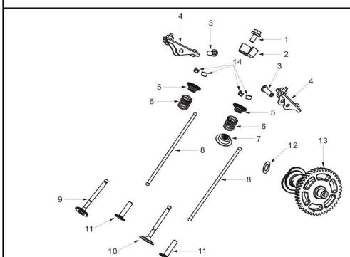
FIG.4 TRAIN,VALVE / CAMSHAFT SUBASSEMBLY (E05)
