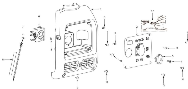
FIG.7 CONTROL PANEL ASSEMBLY/ PANEL HOLDER
