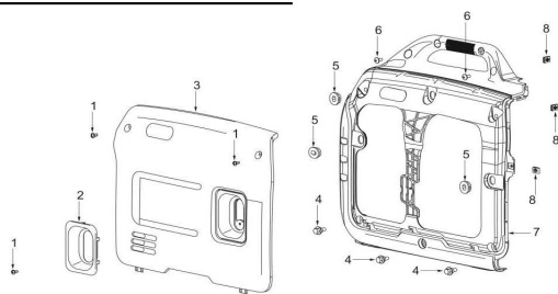
FIG.4: LEFT SHELL
