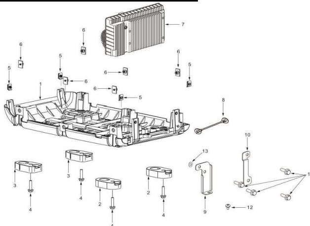
FIG.6: BASE PLATE COMPONENTS/INVERTER
