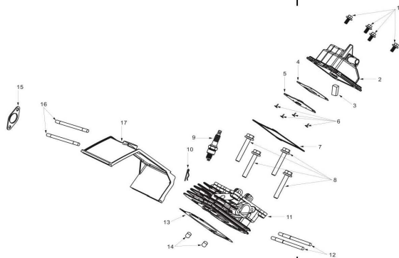
FIG.1 HEAD SUBASSEMBLY, CYLINDER / PLUG,SPARK
