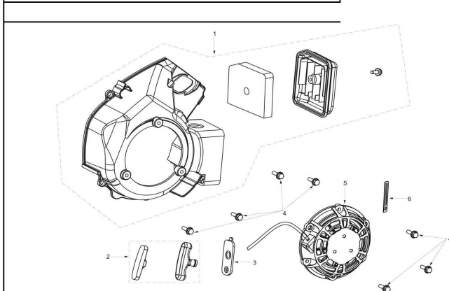
FIG.3 WIND DEFLECTOR ASSEMBLY /PULLER
