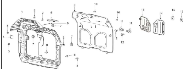
FIG.5: RIGHT SHELL
