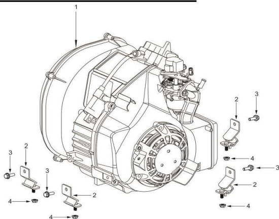
FIG.1 ENGINE
