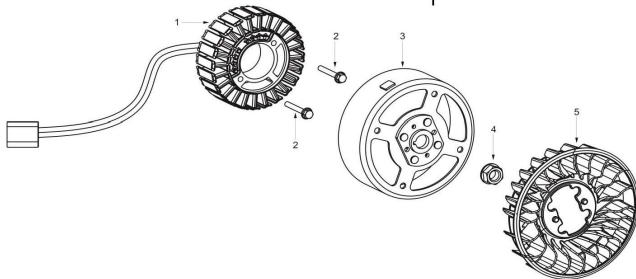
FIG.2 MOTOR ASSEMBLY
